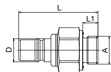
Male Thread with additional Seal
