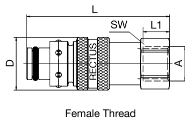
Female Thread
